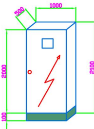
CONTROL CABINET DIMENSIONS
